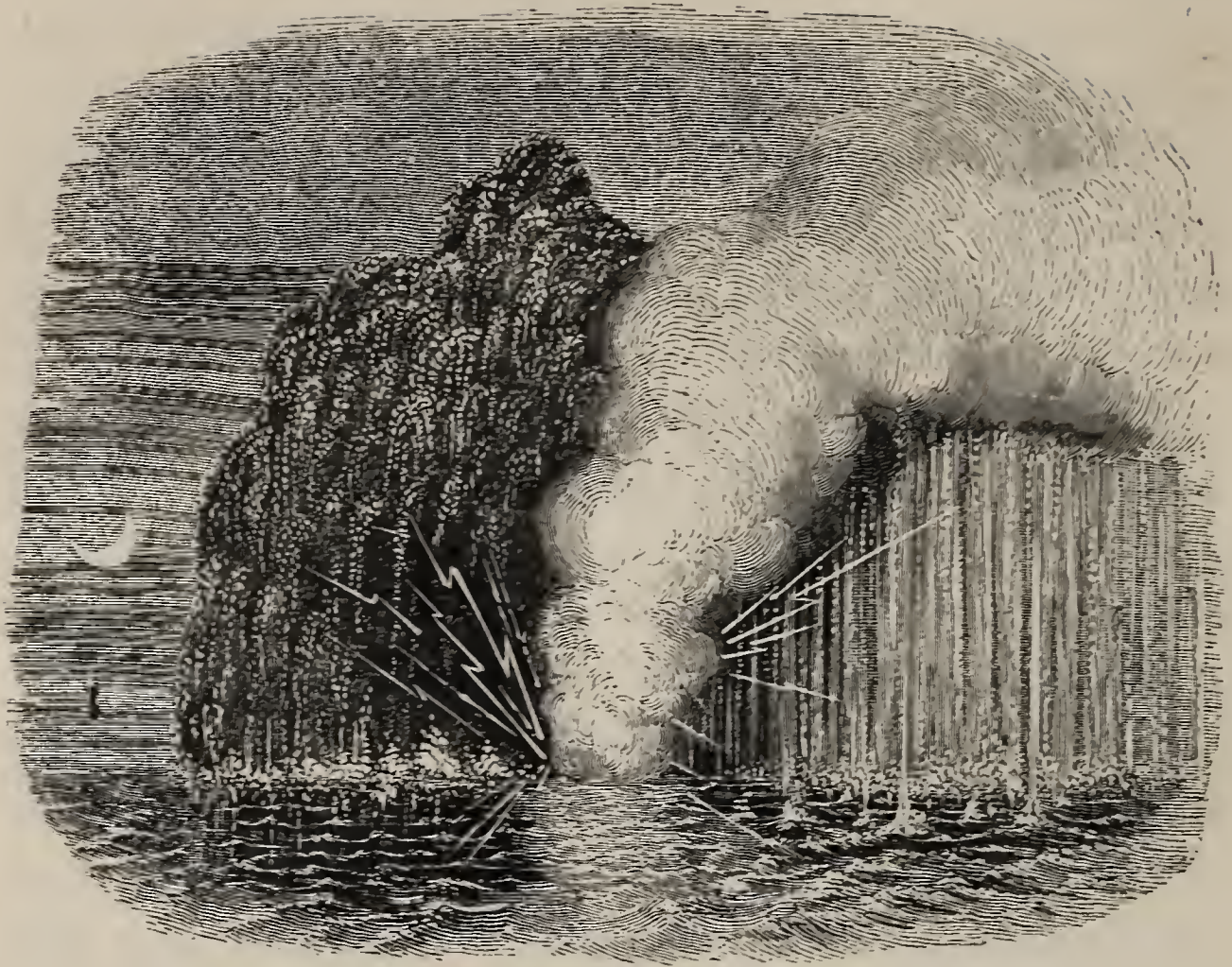
SUBMARINE VOLCANO.
